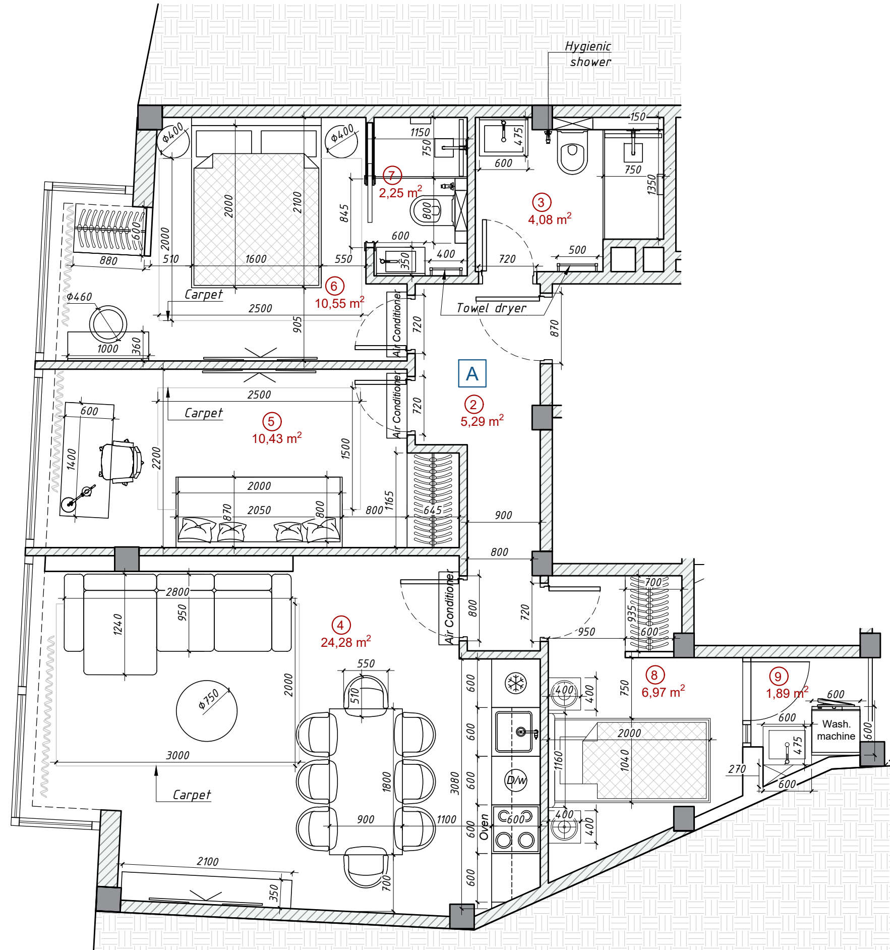
DP - 4 Furniture layout scheme Apartment A
